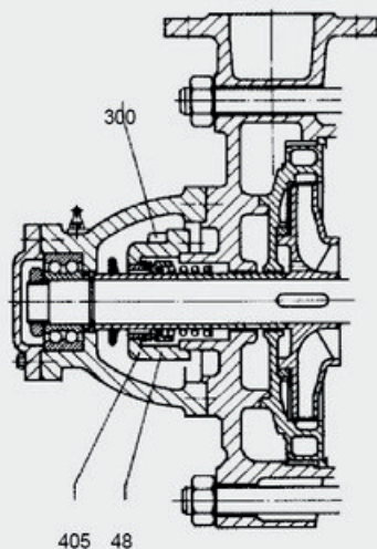
Mechanical Seal Application
