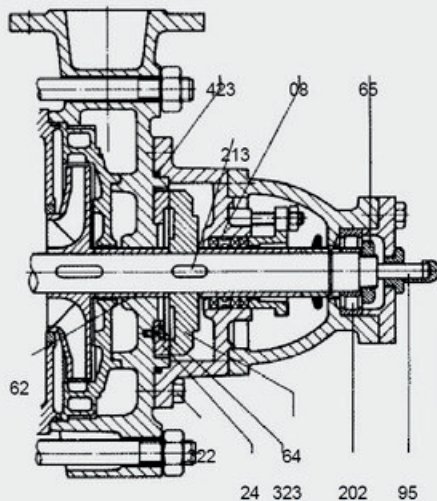
Balance Disc Application (Hm > 200m)
